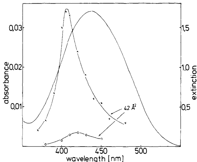
Figure 9. Absorbance spectra of IX: chloroform solution (+ 1% ethanol), c 4.5 \times 10^{-5} mol/L, \lambda_{\max} 435 nm (—). Condensed monolayer on aqueous subphase, a = 42 \text{ \AA}^2/\text{molecule} ; s-polarized light, \lambda_{\max} 420 nm (O-O-O); p-polarized light, \lambda_{\max} 405 nm (x-x-x).
