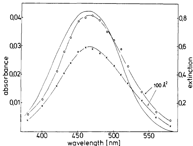
Figure 6. Absorbance spectra of VI: ethanol solution, c = 2.5 \times 10^{-5} mol/L, \lambda_{\max} = 465 nm (—). Monolayer on aqueous subphase, a = 100 \text{ \AA}^2/\text{molecule} , s-polarized light (O-O-O); p-polarized light (x-x-x); \lambda_{\max} = 470 nm.
