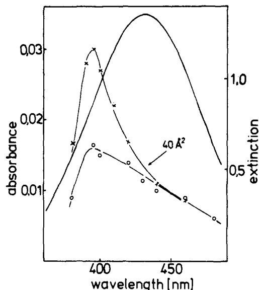
Figure 10. Absorbance spectra of VIII: chloroform solution (+ 1% ethanol), c 4.8 \times 10^{-5} mol/L, \lambda_{\max} 432 nm (—). Condensed monolayer VIII on aqueous subphase, a = 40 \text{ \AA}^2/\text{molecule} ; s-polarized light (O-O-O); p-polarized light \lambda_{\max} 395 nm (x-x-x).
