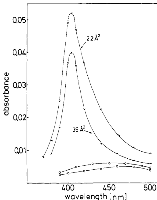
Figure 8. Absorbance spectra of monolayer VI on aqueous subphase for two different surface areas: first condensed state at a = 35 \text{ \AA}^2/\text{molecule} ; second condensed state at a = 22 \text{ \AA}^2/\text{molecule} ; s-polarized light (O-O-O); p-polarized light, \lambda_{\max} = 405 nm (x-x-x).
