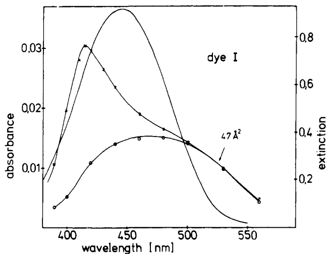
Figure 7. Absorbance spectra of I: cyclohexane solution, c = 3.1 \times 10^{-5} M, \lambda_{\max} = 443 nm (—); monolayer on pure water a = 47 \text{ \AA}^2 , s-polarized light (O-O-O); p-polarized light (x-x-x).
